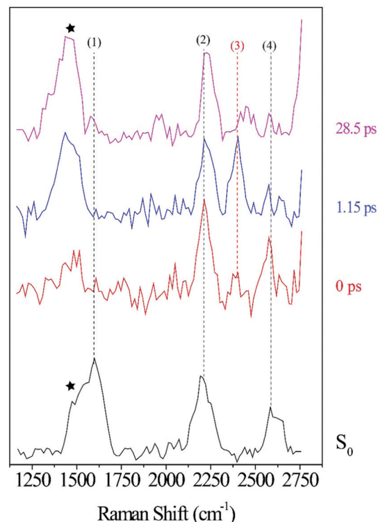
Fig. 5 ODIBO FSRS spectra after 321 nm excitation at 0, 1.15 and 28.5 ps delay-times with peaks at 2206, 2399 and 2578 cm −1 at 0 ps labeled (2), (3), and (4), respectively. The ground state spectrum (black) without actinic excitation is also provided with 1601, 2206 and 2582 cm −1 peaks labeled (1), (2) and (4) respectively. The black stars denote a methanolic peak at 1483 cm −1 .
