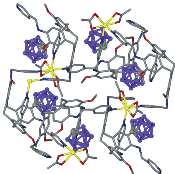
Fig. 2 Section of the crystal structure of [Cd(L5)(OAc) 2 ] showing formation of 2D network and host-guest binding of C 2 B 10 H 12 o-carborane guests (purple). Hydrogen atoms excluded. 44
