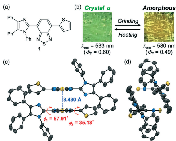
Fig. 1 (a) Molecular structure of 1 . (b) Photographs of the MCL of 1-α ( \lambda_{\text{ex}} = 365 nm). (c) Front view and (d) side view of 1-α for the two molecules in spatial proximity with thermal ellipsoids at 50% probability. All hydrogen atoms are omitted for clarity. Color code: gray = C; blue = N; yellow = S.
