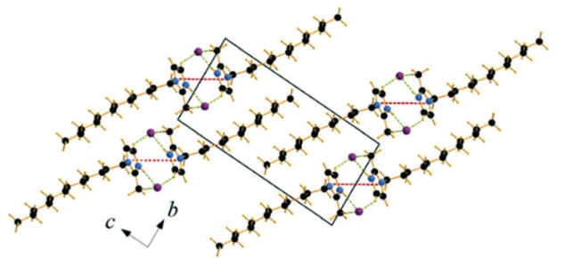
Fig. 5 Packing diagram of \text{C}_{12}\text{C}_1\text{C}_0 . Projection on the bc plane. \text{C}_g - \text{C}_g contacts are shown by red and \text{Br}\cdots\text{H} bonds by green dashed lines.
