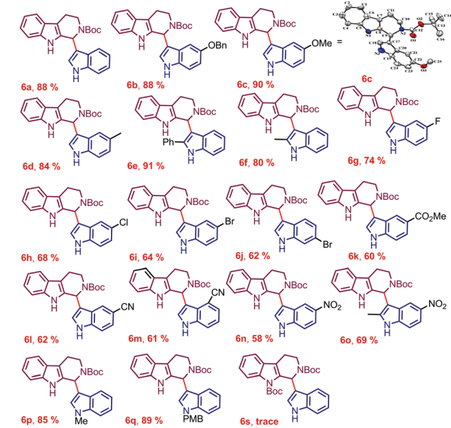
Scheme 1 Substrate scope (synthesis of derivatives of 6a ). a,b a Reaction conditions: tetrahydro- \beta -carboline 1a – c (0.185 mmol, 1.0 equiv.), Trityl salt (0.222 mmol, 1.2 equiv.), indoles 2a – q (0.204 mmol, 1.1 equiv.), and DCM (3.0 mL, 0.06 M), 30 seconds. For substrates 2e and 2f , the reaction time is 10 seconds after the addition of indole. b Isolated yields.
