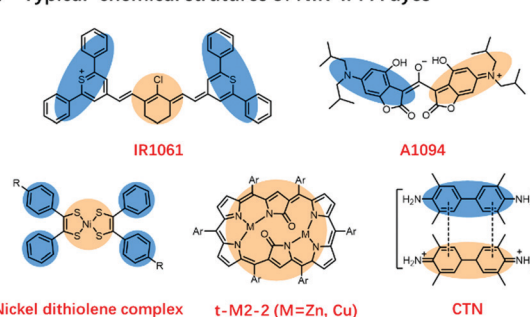
Fig. 2 (a) Typical chemical structures of NIR-I PA dyes. (b) Typical chemical structures of NIR-II PA dyes.
