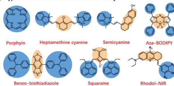
(b) Typical chemical structures of NIR-II PA dyes
