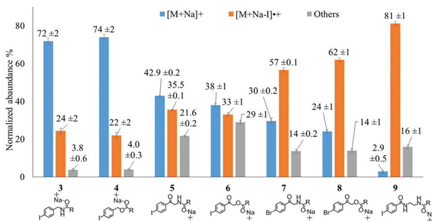
Fig. 4 Analysis of the PD266 photo-conversion of FA 18:1(9Z) as derivatives 3–9. All PD266 mass spectra were acquired via direct infusion of a methanolic solution of the compound with the bars representing the mean normalized ion counts over 80 individual scans and the error bars representing one standard deviation in the mean.
