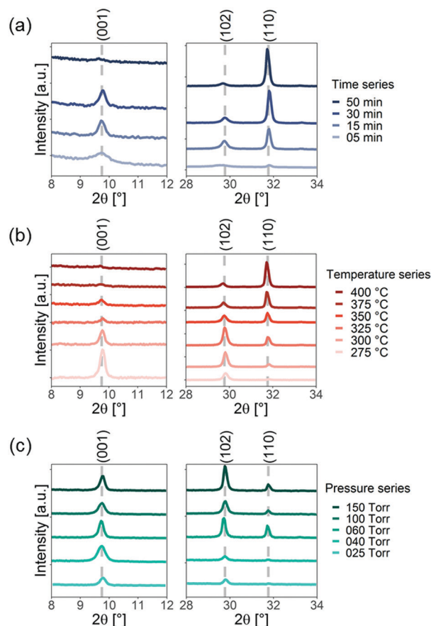
Fig. 2 X-ray diffraction pattern of bismuth oxyiodide grown by chemical vapor deposition (a) during different growth times, (b) at different growth temperatures (where T_{\text{sub}} = T_p + 30^\circ\text{C} ) and (c) different growth pressures. Note that the scales of the vertical axes are different for visualization purposes. The full XRD patterns can be found in Fig. S5, ESI.†
