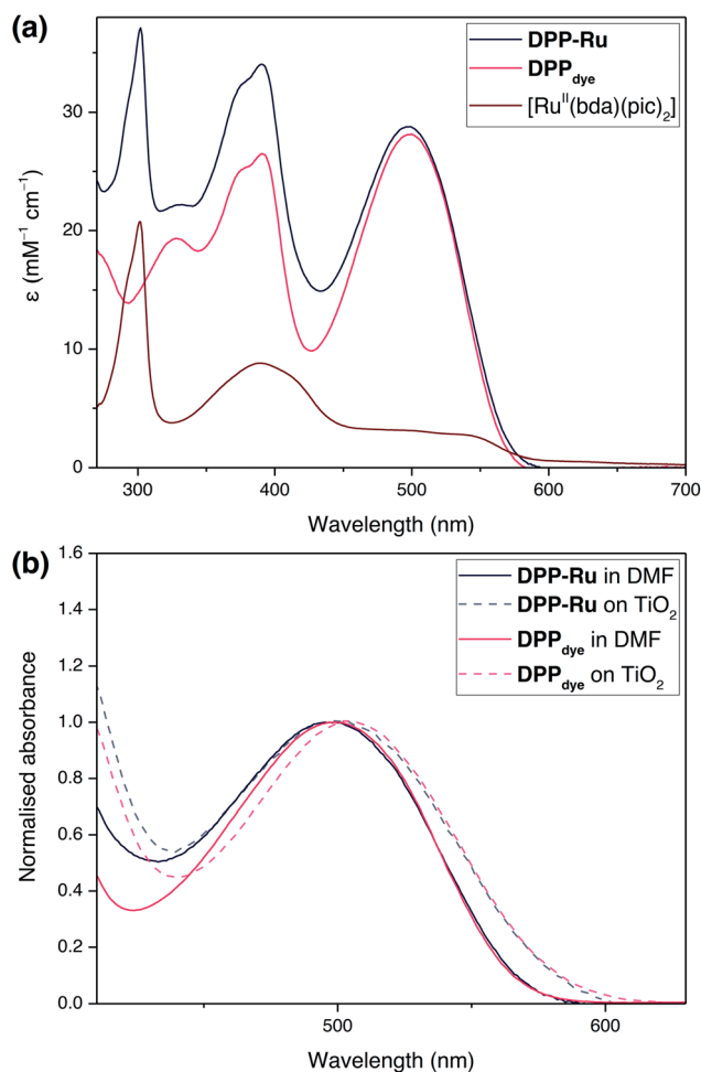
Fig. 2 (a) UV-vis absorption spectra of DPP dye , [\text{Ru}^{\text{II}}(\text{bda})(\text{pic})_2] and DPP-Ru in DMF solution. (b) Normalised UV-vis spectra of DPP dye and DPP-Ru on a \text{mTiO}_2 film coated on a glass slide, and in DMF solution.
