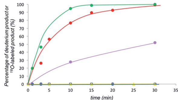
Fig. 2 Generation of deuterated substrates in eqn (4), green: i -Pr 2 NEt and p -nitrophenol, red: pyrrolidine and p -nitrophenol, blue: p -nitrophenol, yellow: i -Pr 2 NEt, and generation of 18 O labelled substrate in eqn (5), purple.
