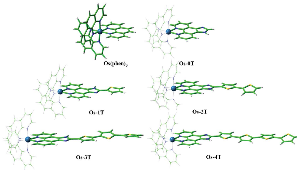
Fig. 3 Optimized geometries of reference compound [\text{Os}(\text{phen})_3]^{2+} and \text{Os-}n\text{T} ( n = 0-4 ) in a water environment at the PBE0/6-31+G**/SDD level of theory.
