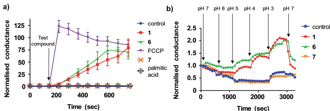
Fig. 3 Aryl-ureas and the protonophore FCCP modulate proton conductance in tethered lipid bilayer membranes. (a) Addition of active aryl ureas 1 and 6 (10 \mu M) and FCCP (0.5 \mu M) increased conductance across a DOPC lipid bilayer tethered to a gold electrode, as measured by electrical impedance spectroscopy. The inactive aryl urea 7 (10 \mu M) and protein-dependant uncoupler palmitic acid failed to increase bilayer conductance. Data normalised to baseline control. (b) Sequential reduction of membrane pH leads to an increase in relative membrane conductivity for active aryl ureas 1 and 6 (10 \mu M). For the inactive aryl urea 7 (10 \mu M) there was no relative conductance increase. Data normalised to conductance of aryl-urea treated membranes at pH = 7. Data represents the mean \pm SEM of 3 independent experiments.
