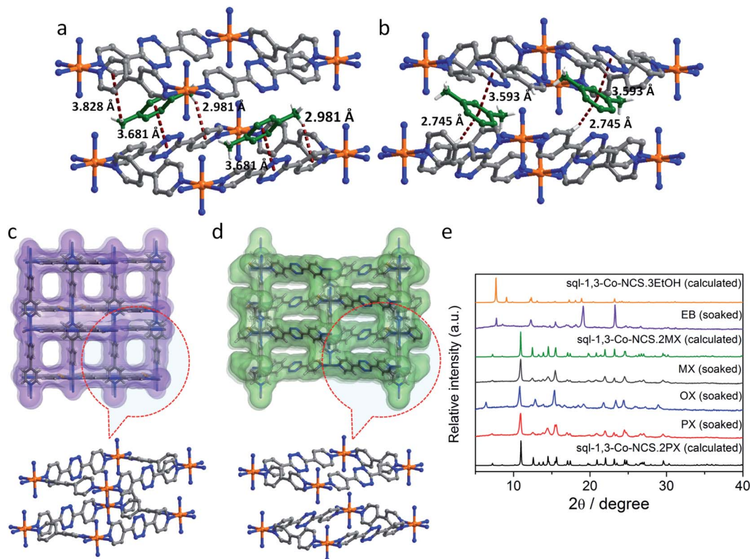
Fig. 6 (a and b) Host–guest interactions in the PX and MX loaded phases, respectively; (c and d) the Connolly surfaces of sq1-1,3-Co-NCS·3EtOH and sq1-1,3-Co-NCS·2PX respectively, with a probe radius of 1.4 Å. (e) PXRD patterns for the solvent soaking experiments in pure xylenes and ethylbenzene.
