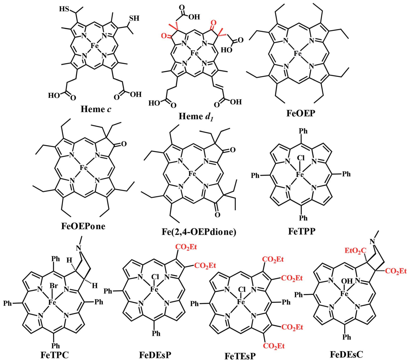
Fig. 3 Structure of the naturally occurring heme and synthetic Fe-porphyrinoids. FeOEP, FeOEPone, and Fe(2,4-OEPdione) were synthesized previously. 32,47,48
