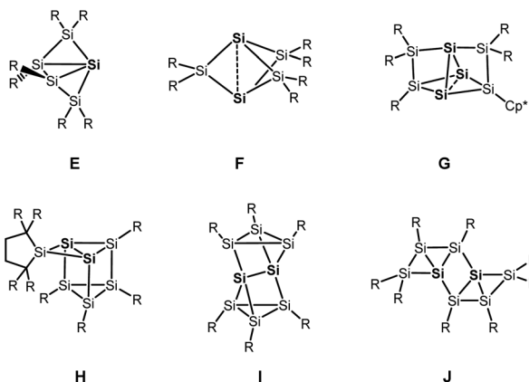
Scheme 2 Other silicon clusters with hemispheroidal silicon atoms (highlighted in bold).
