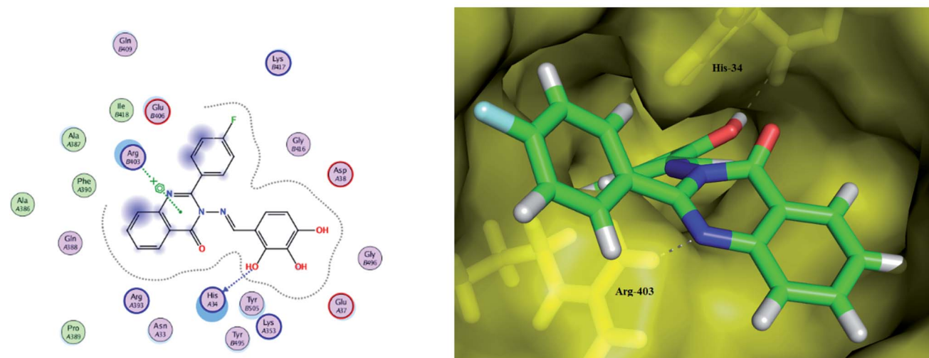
Fig. 5 (a) A 2D animated structure showing the binding interactions between compound Ib and SGp and (b) a 3D representation showing the position of compound Ib within the cavity of SGp.
