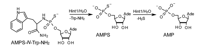
Scheme 3 The HINT1 catalyzed hydrolysis of adenosine-5'- O -(( L -tryptophan amide- N_{\alpha} -yl)-phosphoramidothioate) (AMPS-Trp-NH 2 ), followed by desulfuration of the AMPS intermediate leading to the formation of adenosine-5'- O -phosphate.
