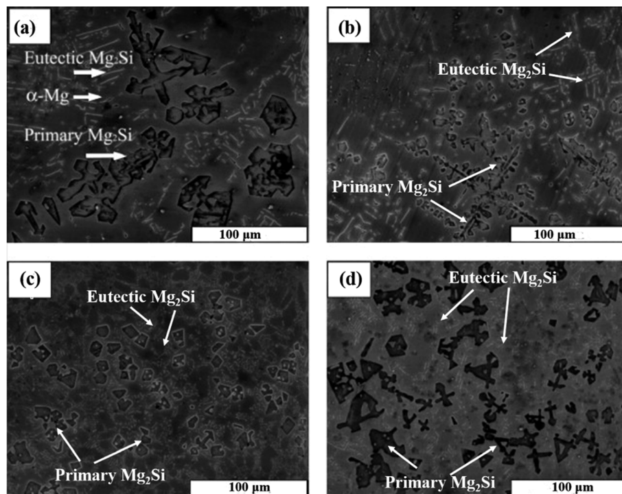
Fig. 7 SEM micrographs of Mg–5 wt% Si alloys (a) without modifier, (b) 5 wt% \text{K}_2\text{TiF}_6 , (c) 5 wt% \text{KBF}_4 and (d) 5 wt% \text{KBF}_4 + \text{K}_2\text{TiF}_6 (mixtures with weight ratio of 4 : 1). This figure has been reproduced from ref. 24 with permission from Elsevier, copyright 2005.
