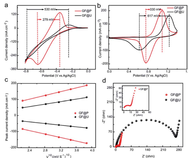
Fig. 4 (a) and (b) Cyclic voltammeteries of \text{V}^{3+}/\text{V}^{2+} and \text{VO}_2^+/\text{VO}_2^+ redox using GF@U and GF@P electrodes at a scan rate of 10 \text{ mV s}^{-1} . (c) The relationship between GF@U and GF@P peak current density and square root of sweep speed. (d) Impedance diagram of GF@U and GF@P.
