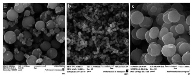
Fig. 25 SEM images of samples with [( \pm )-2-( cis -butyl)aniline] = 0.5 M; (a) without an initiator, (b) with phenylenediamine, and (c) with aniline dimer. Reproduced with permission from ref. 47.
