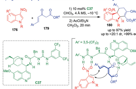
Scheme 40 Organo-CADA oxidation of C2-substituted indoles by Zhang and coworkers. 75
