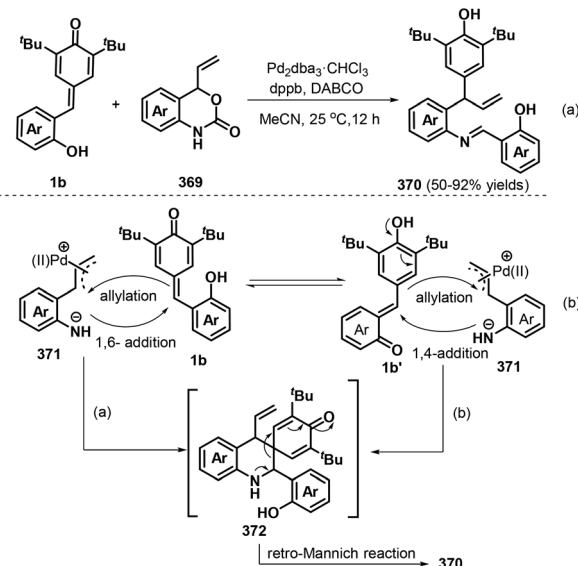
Scheme 84 Catalytic C=C bond cleavage of p -QMs.
