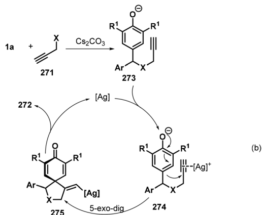
Scheme 60 [3 + 2] annulation toward spirocyclohexadienones.
