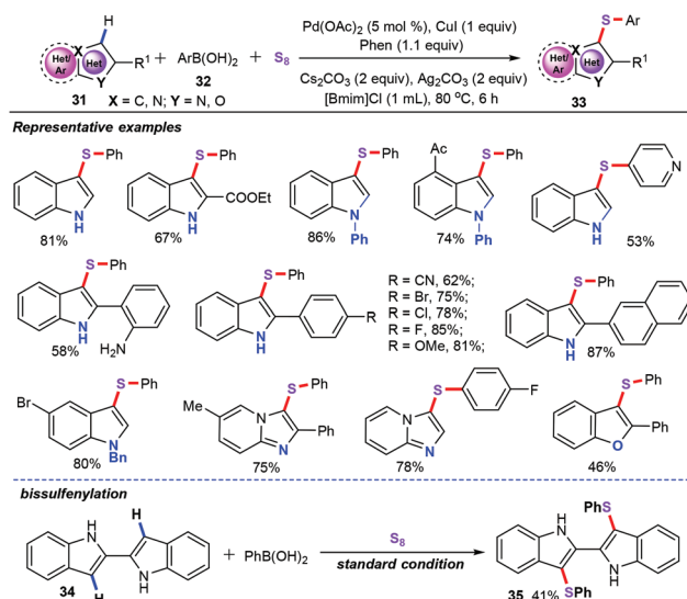
Scheme 13 Palladium-catalyzed oxidative sulfenylation of electron-rich heteroarenes.
