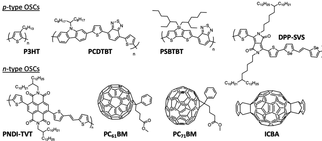
Fig. 5 Chemical structures of P3HT , PCDTBT , PSBTBT , DPP-SVS , PNDI-TV , PC 61 BM , PC 71 BM and ICBA .
