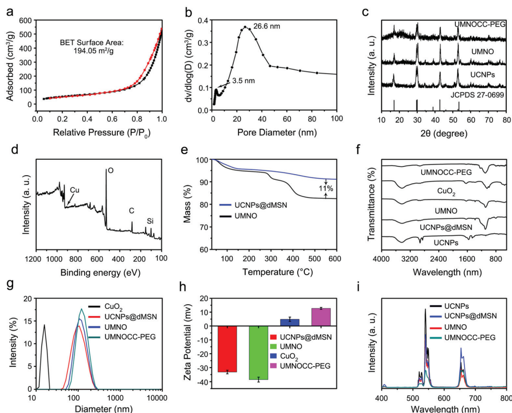
Fig. 2 Characterization of UMNOCC-PEG nanoparticles. (a) N 2 adsorption-desorption isotherms and (b) corresponding pore-size distribution of UCNPs@dMSN. (c) XRD patterns of UCNPs, UMNO, and UMNOCC-PEG. (d) Survey XPS spectra of UMNOCC-PEG and (e) thermogravimetric analysis curves of UCNPs@dMSN and UMNO. (f) FT-IR spectra of UCNPs, UCNPs@dMSN, UMNO, CuO 2 , and UMNOCC-PEG. (g) Particle-size distribution of CuO 2 , UCNPs@dMSN, UMNO, and UMNOCC-PEG. (h) Zeta potential of UCNPs@dMSN, UMNO, CuO 2 , and UMNOCC-PEG. (i) Upconversion emission spectra of UCNPs, UCNPs@dMSN, UMNO, and UMNOCC-PEG.
