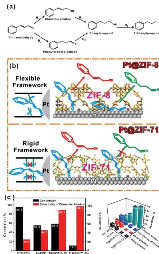
Fig. 12 (a) Reaction paths of CAL hydrogenation. (b) Schematic illustration of hydrogenation of CAL on Pt NPs embedded within flexible ZIF-8 and rigid ZIF-71, respectively. (c) Conversions and selectivity of four products of CAL hydrogenation over Pt/C-20%, Pt-PVP, Pt@ZIF-8-1%, and Pt@ZIF-71-1%. Reproduced with permission. 75 Copyright©2017 WILEY-VCH Verlag GmbH & Co. KGaA.
