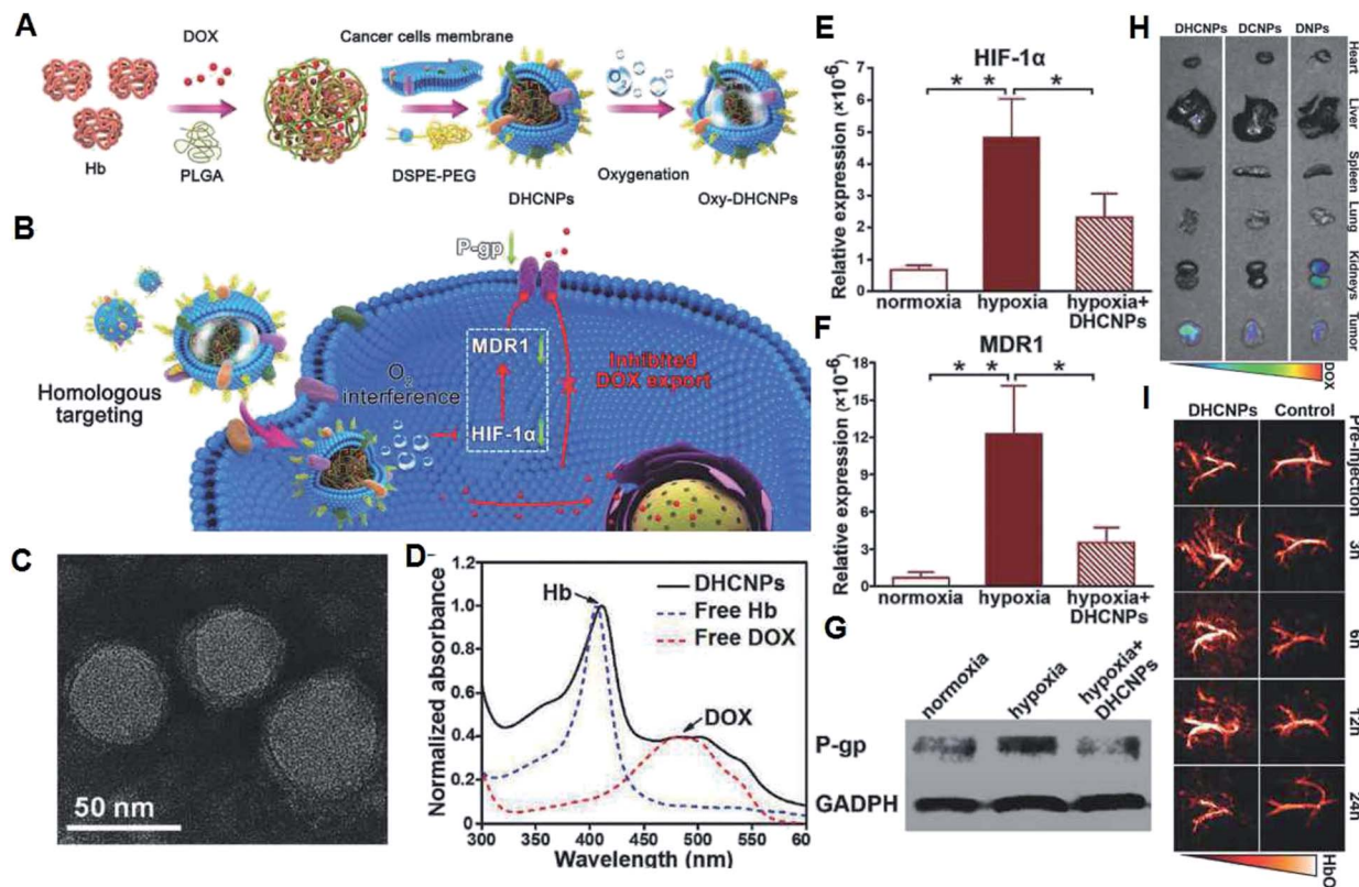
Fig. 4 (A) Synthesis of oxy-DHCNPs. (B) Schematic illustration of the therapeutic mechanisms of DHCNPs. (C) TEM image of DHCNPs. (D) UV-Vis absorption spectra of different solutions. (E–G) Contents of HIF-1 \alpha , MDR1, and P-gp of MCF-7 cells treated with DHCNPs. (H) FL images of normal organs and tumors of tumor-bearing mice after injection of different solutions. (I) PA images of tumors after the injection of DHCNPs. 32
