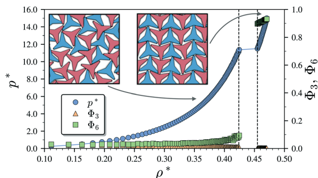
Fig. 2 Pressure–density ( P^*-\rho^* ) phase diagram of the repulsive model of 1024 non-convex hexagonal platelets. The dependence of the global orientational order parameters \Phi_3 and \Phi_6 on the density is also indicated. The snapshots in the insets are representative configurations for the isotropic (left) and striped crystal phase with the pmg symmetry group (right), respectively. The particles are represented by the convex envelop of the rigid polybead model and the two different colours (shades) are used to represent opposite orientations. Vertical dashed lines indicate phase boundaries.
