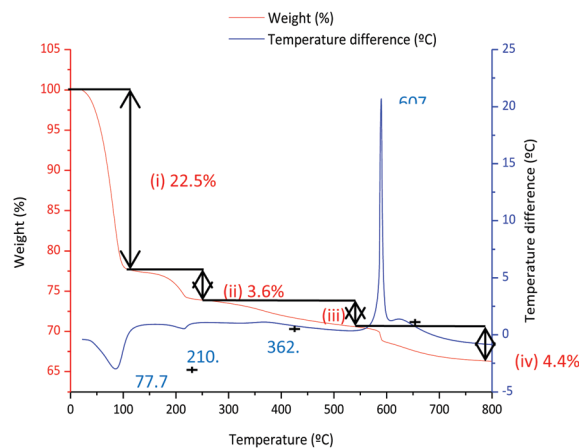
Fig. 5 TGA and DTA analysis of the 80\text{ }^\circ\text{C} -12 h dried 80\text{SiO}_2 : 20\text{LaF}_3 particulate sol.
