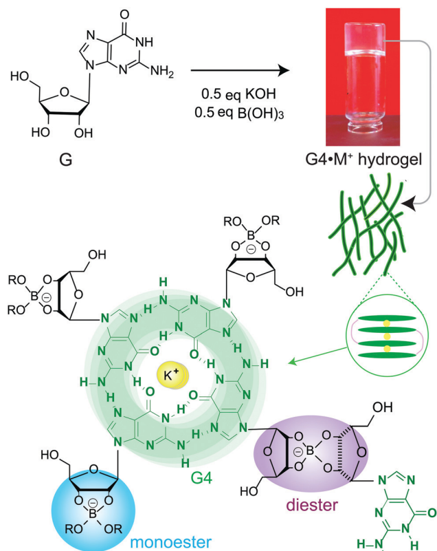
Scheme 1 Schematic diagram of the gelation mechanism of G4 \cdot M^+ ( M^+ = K^+, Na^+ ) hydrogels upon mixing guanosine (G) with metal borate salts. Guanosine borate cis diesters favour gelation by covalently cross-linking stacked G -quartets.
