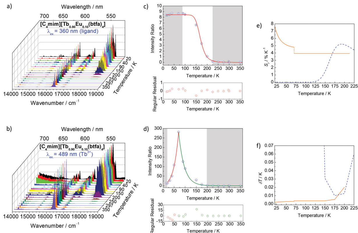
Fig. 6 Emission spectra of the [\text{C}_4\text{mim}][\text{Tb}_{0.90}\text{Eu}_{0.10}(\text{btfa})_4] complex recorded as a function of temperature with excitation at 360 nm (a) and 489 nm (b). In (a) the emission spectra are normalized by the intensity at 611 nm ( ^5\text{D}_0 \rightarrow ^7\text{F}_2 ), while in (b) they are normalized by the maximum intensity in each individual spectrum. The ^5\text{D}_4 \rightarrow ^7\text{F}_5/{}^5\text{D}_0 \rightarrow ^7\text{F}_2 ratios measured with 360 and 489 nm are shown in (c and d), respectively. The lines represent the fits using eqn (5) and (6), respectively. The residual plot is shown on the bottom for a judgment of the fit quality. The shadowed areas mark the regions in which the thermometric parameters change within its uncertainty meaning that for these temperatures the thermometer is out of the so-called operating range. Relative thermal sensitivity (e) and temperature uncertainty (f) obtained at 360 nm (dashed line) and 489 nm (solid line). In (f), the temperature range is limited to \delta T < 0.07 K.
