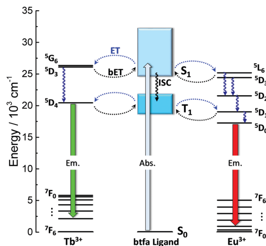
Fig. 7 Schematic partial energy level diagram of the [\text{C}_4\text{mim}][\text{Tb}_{1-x}\text{Eu}_x(\text{btfa})_4] ( x = 0.01, 0.05 and 0.10 ) complexes involving the btfa ligand, \text{Eu}^{3+} and \text{Tb}^{3+} electronic states. T_1 is the lowest ligand triplet level and S_0 and S_1 are the ligand ground and lowest singlet excited states, respectively. Abs. is the initial absorption, ISC is the intersystem crossing and Em is the emission. ET and bET are the forward and backward energy transfer, respectively.
