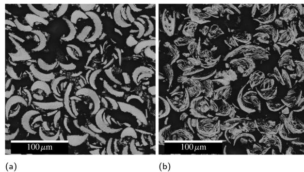
Fig. 8 Cross-sectional electron micrographs of syringe-printed PVD particles (a) as printed and (b) after reaction. The black background is mounting epoxy.
