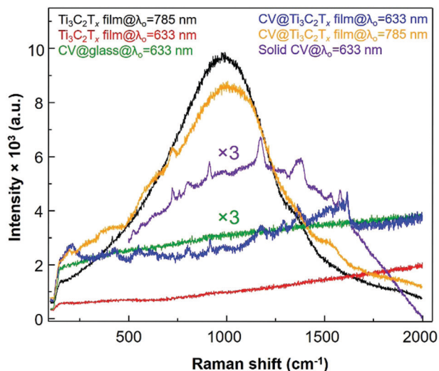
Fig. 5 The normal Raman spectra (ca. 12.732 \text{ ng cm}^{-2} of CV on bare glass and surface-enhanced Raman scattering (SERS) of CV dye molecules (ca. 12.732 \text{ ng cm}^{-2} ) adsorbed on \text{Ti}_3\text{C}_2\text{T}_x film@glass with excitation laser wavelengths of both 633 nm and 785 nm.
