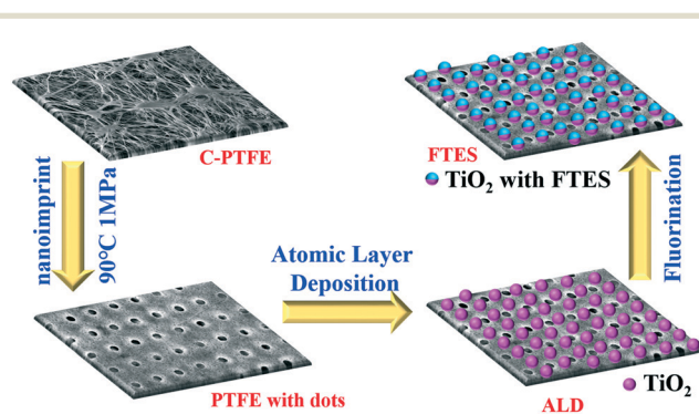
Fig. 1 Schematic illustration of design and procedures for fabricating the nanoimprint PTFE membrane with a fluorinated TiO 2 deposition layer.
