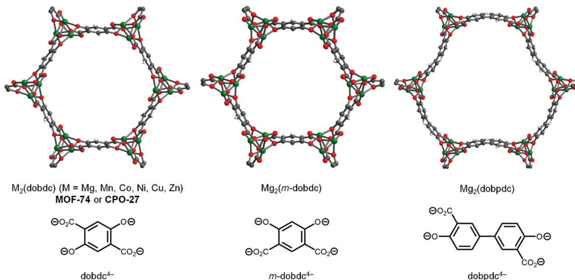
Fig. 1 Structures of the open metal site metal–organic frameworks M_2(\text{dobdc}) (M = Mg, Mn, Co, Ni, Cu, Zn; \text{dobdc}^{4-} = 2,5-dioxidobenzene-1,4-dicarboxylate), Mg_2(m\text{-dobdc}) ( m\text{-dobdc}^{4-} = 2,4-dioxidobenzene-1,5-dicarboxylate), and Mg_2(\text{dobpdc}) ( \text{dobpc}^{4-} = 4,4'-dioxidobiphenyl-3,3'-dicarboxylate). The cross-pore diameters in these MOFs are 15.4 Å, 14.9 Å, and 22.8 Å, respectively. Gray, white, red, and green spheres represent carbon, hydrogen, oxygen, and magnesium, respectively.
