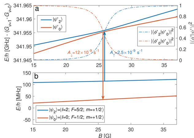
Fig. 12 (a) Adiabatic level energies, E , as a function of the magnetic field, B , showing an avoided crossing between two states originating from |I'=2, F'=3/2, m'=-3/2\rangle ( |\psi_2'\rangle , blue line) and |I'=0, J'=3/2, m'=-3/2\rangle ( |\psi_0'\rangle , red line) in the v'=1, N'=2 rovibrational-state manifold. The dashed-dotted lines indicate the degree of mixing, |\langle\phi_2'|\psi_0'\rangle|^2 , where |\phi_j'\rangle are the basis states ( j=0, 2 ) describing |\psi_j'\rangle at low magnetic fields. At a magnetic-field strength of \sim 25.8 \text{ G} , a 50–50 mixture of the I=0 and I=2 states is predicted. (b) Levels of the I=2 (blue) and the I=0 (red) nuclear-spin configurations in the rovibrational ground state are coupled by a resonant two-photon process (arrows). The coupling is performed through S(0) transitions to one of the highly mixed nuclear-spin states. The coupling strengths to the |\psi_0'\rangle state in the form of the Einstein A coefficients for \Delta m = -2 transitions are given in the plot.
