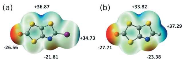
Fig. 3 Molecular electrostatic potential surfaces mapped at 0.001 e ^{-} au ^{-3} isodensity surface for (a) 2 ; (b) 3 . The common color scale ranges from −28 kcal mol ^{-1} (red) to +40 kcal mol ^{-1} (blue).
