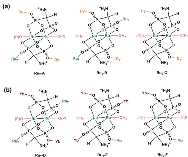
Scheme 3 Coordination modes of \text{Ru}_2(\text{H}_x\text{ampd})_2 dimers in 17 (a) and 18 (b). Reprinted with permission from ref. 24. Copyright 2019, American Chemical Society.
