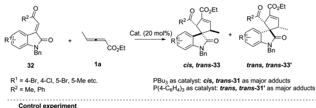
Scheme 9 Phosphine-catalysed stereoselective dearomatization of 3- \text{NO}_2 -indoles.
