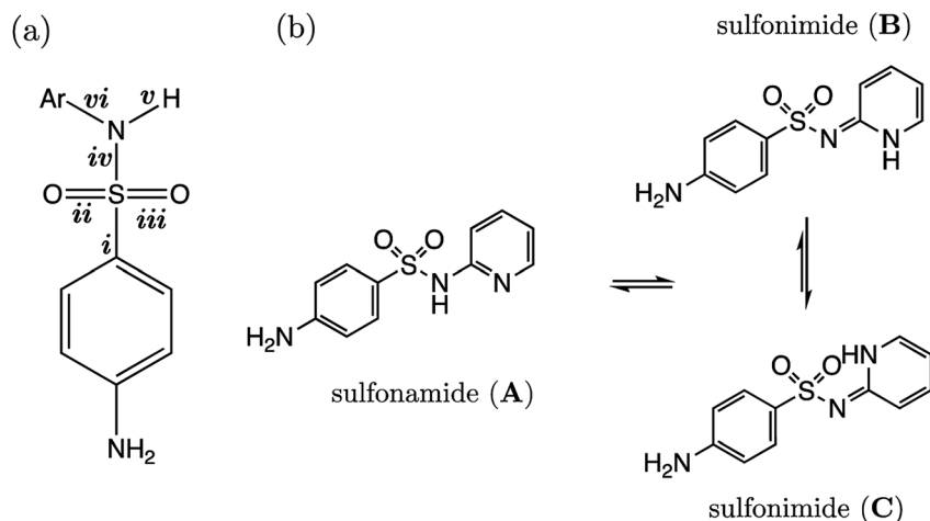
Fig. 6 (a) Common fragment of all sulfanilamides considered as part of the S2 (AP-BSA) reaction series with studied bond lengths labelled i – vi ; (b) two tautomeric forms are available to 4-amino- N -(2-pyridyl)benzenesulfonamides (NHAS), which are shown as sulfonamide (A), and the two conformational isomers of the same tautomer, sulfonimides (B) and (C).
