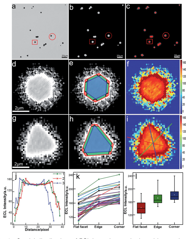
Fig. 2 Spatial distribution of ECL intensity on single gold nanoplates. (a) Bright-field image, (b) ECL image (exposure time: 200 ms) and (c) false-color overlay of the bright-field and ECL images. (d and g) Magnified areas of the ECL image (b) marked by a red circle and square. (e and h) Divided regions of corners (red), edges (green), and the flat surface facet (blue) in the ECL images of (e and h). (f and i) 2D spatial distribution ECL intensity obtained by using Matlab. (j) ECL intensity gradients at three measuring lines marked in (i). (k) Statistical site-specific ECL intensity of 35 nanoplates. (l) Box charts of the ECL intensities from corner, edge and flat facet regions.
