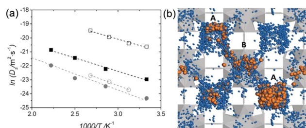
Fig. 23 (a) Arrhenius plot of D_s for protons (squares) and water molecules (circles) in the fully hydrated \text{UiO-66}(\text{Zr})-(\text{CO}_2\text{H})_2 : QENS (open symbols) and aMS-EVB3-MD simulations (full symbols). (b) Illustration of simulation result for the water (blue)-mediated pathway with proton (orange) along the tetrahedral (A) and octahedral cages (B) of \text{UiO-66}(\text{Zr})-(\text{CO}_2\text{H})_2 at 450 K. Reproduced from ref. 81 with permission from Wiley-VCH, Copyright 2016.
