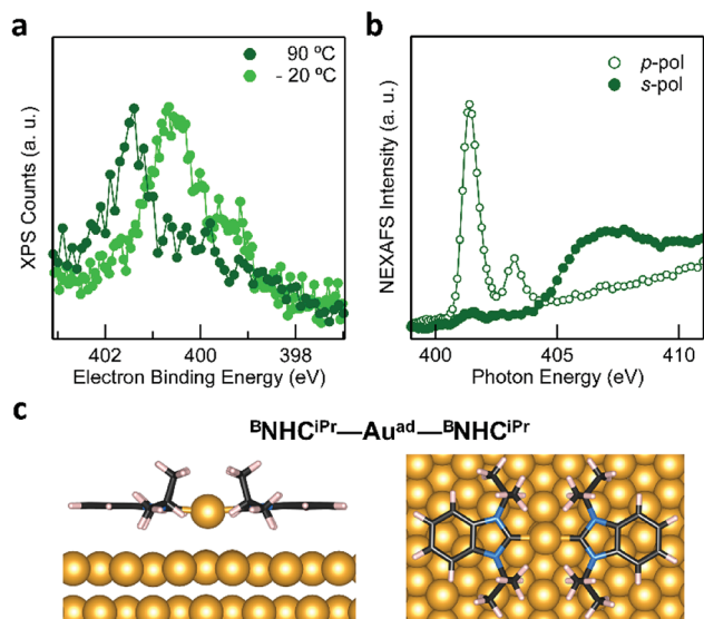
Fig. 4 (a) XPS N 1s spectra of a {}^{\text{B}}\text{NHC}^{\text{iPr}} monolayer deposited on a cold substrate at -20\text{ }^{\circ}\text{C} (light green), and then annealed to 90\text{ }^{\circ}\text{C} (dark green). The broad peak in the low-temperature spectrum comprises different components likely due to multiple molecular adsorption sites and/or of second-layer molecules. Thermal annealing generates a single sharp N 1s peak shifted to higher binding energy by \sim 1\text{ eV} . (b) NEXAFS spectrum collected at the N K-edge for the {}^{\text{B}}\text{NHC}^{\text{iPr}} monolayer annealed to 90\text{ }^{\circ}\text{C} : a strong dichroism is clearly visible. The \text{N } 1\text{s} \rightarrow \pi^*\text{-LUMO} resonance is strongly enhanced in p-pol indicating that the molecules lie nearly flat on the surface. (c) DFT-optimized energy minimum structure of a {}^{\text{B}}\text{NHC}^{\text{iPr}}\text{-Au}^{\text{ad}}\text{-}{}^{\text{B}}\text{NHC}^{\text{iPr}} complex adsorbed on an Au(111) 5 \times 7 slab. Note that the adatom is above a hollow site on the Au(111) surface.
