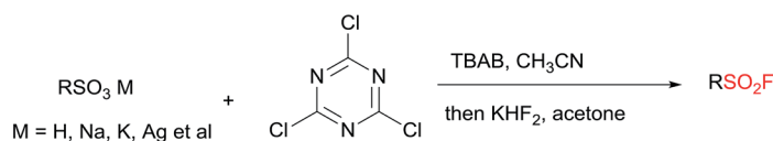
Scheme 1 Strategies for the assembly of sulfonyl fluorides.
