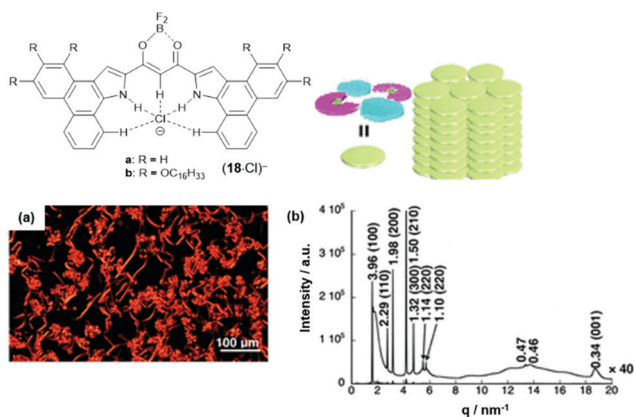
Fig. 18 Schematic representation of the phenanthro[b]-fused \pi -electronic anion ( 18-Cl ) - . (a) POM image of ( 14a )( 18b-Cl ) at 180 °C upon cooling. (b) Synchrotron XRD pattern of ( 14a )( 18b-Cl ) at 150 °C upon cooling; the proposed supramolecular packing mode of the assembly is also shown. 56 Figure reproduced with kind permission; © 2019 American Chemical Society.
