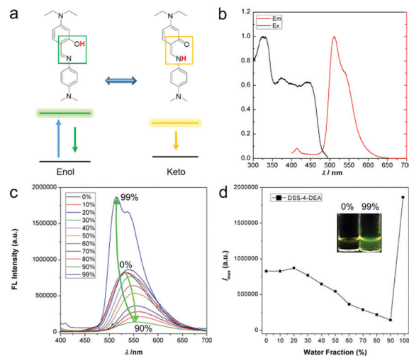
Fig. 1 4- N,N -Dimethylaminoaniline salicylaldehyde Schiff-base (DSS) ESPT molecules with different substituents.
