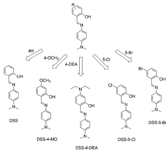
Scheme 1 4- N,N -Dimethylaminoaniline salicylaldehyde Schiff-base (DSS) ESPT molecules with different substituents.
