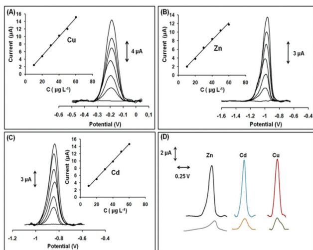
Fig. 9 SWASV voltammograms and respective calibration plots in the range 10\text{--}60\ \mu\text{g L}^{-1} (step: 10\ \mu\text{g L}^{-1} ) of (A) \text{Cu}^{2+} in 0.1\ \text{mol L}^{-1} acetate buffer, (B) \text{Zn}^{2+} in 1 \times 10^{-3}\ \text{mol L}^{-1} KCl, and (C) \text{Cd}^{2+} in 0.1\ \text{mol L}^{-1} acetate buffer (pH 4.5). (D) SWASV voltammograms of 30\ \mu\text{g L}^{-1} of \text{Zn}^{2+} , \text{Cd}^{2+} , \text{Cu}^{2+} (black, blue, and red lines, respectively) obtained with the modified GPE with Ca-MOF and SWASV voltammograms of 30\ \mu\text{g L}^{-1} of \text{Zn}^{2+} , \text{Cd}^{2+} , and \text{Cu}^{2+} (gray, orange, and green lines, respectively) obtained with the bare GPE. Reproduced from ref. 78a with permission from the Royal Society of Chemistry.
