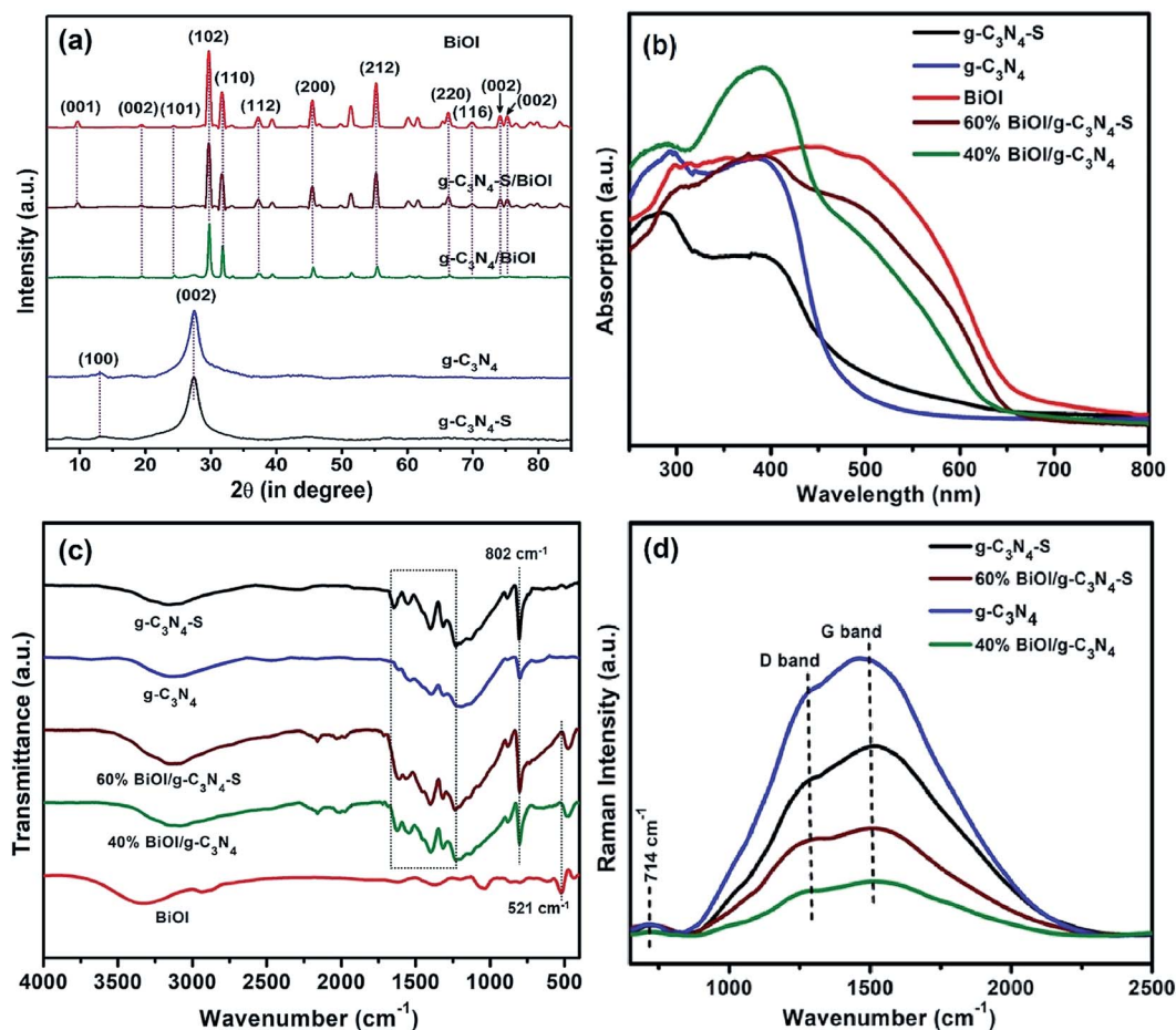
Fig. 4 (a) X-ray diffractograms of pristine BiOI, \text{g-C}_3\text{N}_4\text{-S/BiOI} , \text{g-C}_3\text{N}_4\text{/BiOI} composites, pristine \text{g-C}_3\text{N}_4 (blue) and pristine \text{g-C}_3\text{N}_4\text{-S} (black) (b) UV-Vis absorption spectra collected in DRS mode (c) FTIR transmission spectra of pristine \text{g-C}_3\text{N}_4\text{-S} , pristine \text{g-C}_3\text{N}_4 , \text{g-C}_3\text{N}_4\text{-S/BiOI} , \text{g-C}_3\text{N}_4\text{/BiOI} and pristine BiOI (d) Raman spectra ( \lambda_{\text{exc}} = 780 \text{ nm} ) of pristine \text{g-C}_3\text{N}_4\text{-S} , pristine \text{g-C}_3\text{N}_4 , \text{g-C}_3\text{N}_4\text{-S/BiOI} and \text{g-C}_3\text{N}_4\text{/BiOI} heterostructures. Color: BiOI (red), \text{g-C}_3\text{N}_4\text{-S/BiOI} (wine red), \text{g-C}_3\text{N}_4\text{/BiOI} (green) and \text{g-C}_3\text{N}_4\text{-S} (black).
