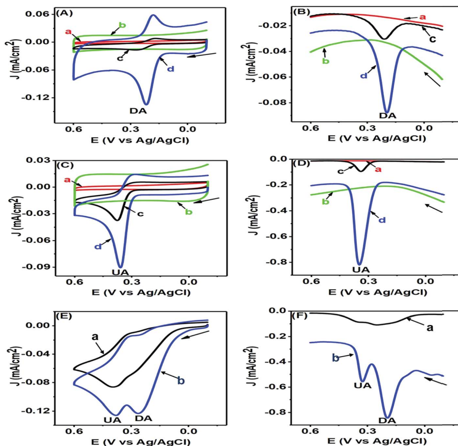
Fig. 7 (A) CVs and DPVs (B) of blank 0.1 M PBS solution of pH 7.0 (a and b) and 50 \mu M DA (c and d) in the same PBS of pH 7.0 at the GCE (a and c) and PTPCNs/GCE (b and d). CVs (C) and DPVs (D) of blank 0.1 M PBS of pH 7.0 (a and b) and 200 \mu M UA (c and d) in PBS of pH 7.0 at the GCE (a and c) and PTPCNs/GCE (b and d). CVs (E) and DPVs (F) of the mixture of 50 \mu M DA and 200 \mu M UA in 0.1 M PBS of pH 7.0 at the bare GCE (a) and PTPCNs/GCE (b).
