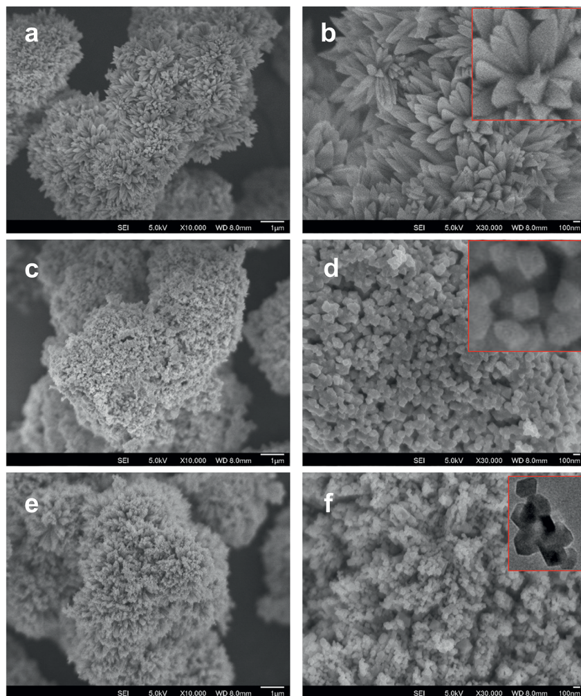
Fig. 2 SEM images: (a and b) [Co/Ni][OH] 2 , (c and d) Co 3 O 4 /NiO-400 °C, (e and f) Co 3 O 4 /NiO-600 °C microsphere composites at low and high magnifications. Scale bars: 1 μm in a, c, e; 100 nm in b, d, f.
